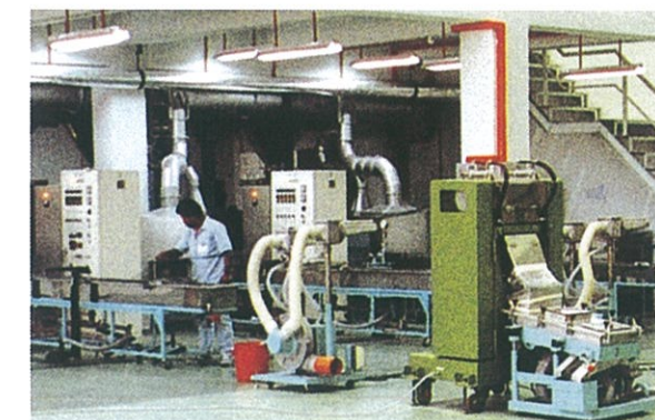
Extrusion Line
